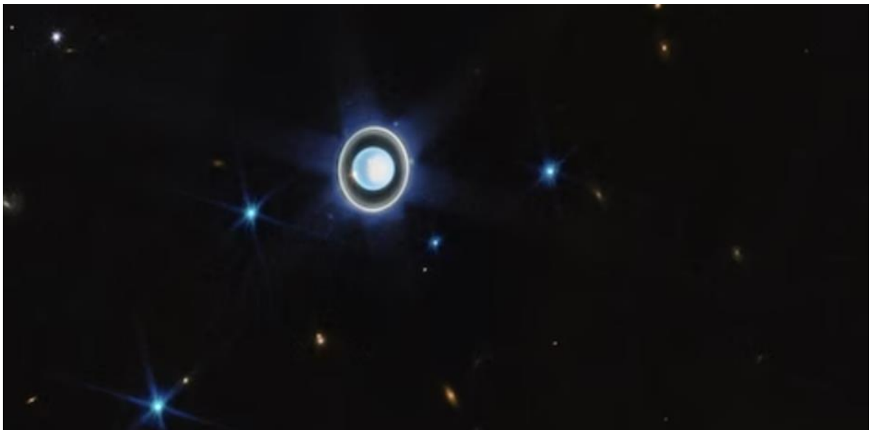
James Webb Telescope image of Uranus with its moons
