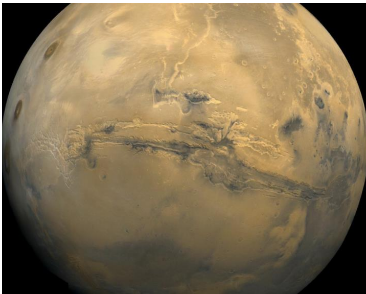
Mars with its mighty gash or blow
