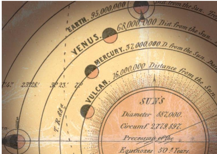
Planet Vulcan Lithograph Map from 1846
